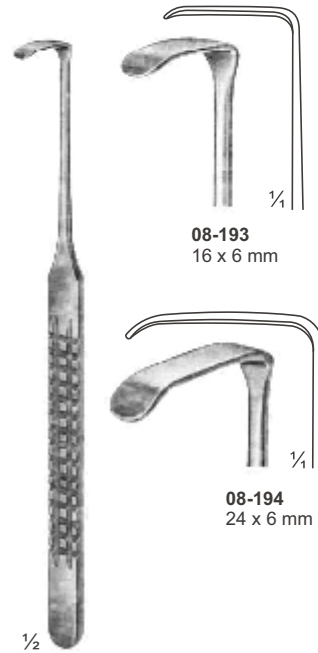
08-193 - 194 LANGENBECK-GREEN 160 mm
