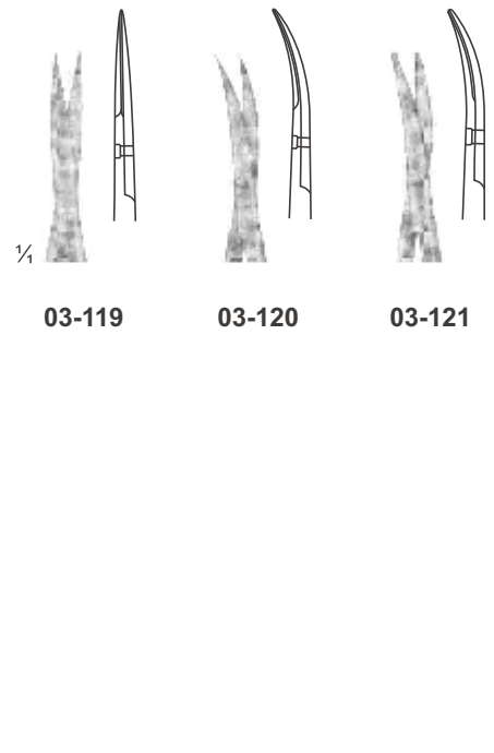
03-119 - 121 Micro Dissecting Scissor Size: 145 mm
