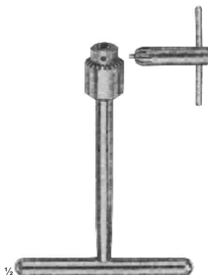
23-155 Drilling chuck, cannulated, for shanks up to 4.5 mm diam., And for triangular shaft width across flats 4.7 mm
